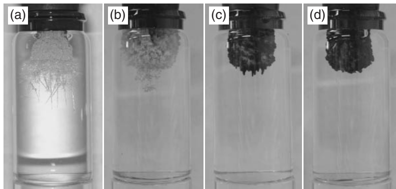
Fig. 2. The photographs of the silver dendrites after 2 h reaction. (a) the outside of the bore tube (the control < 0.0005 T), (b) the bottom position (9.8 T, +1070 T 2 /m), (c) the middle position (15.0 T, +50 T 2 /m), (d) the top position (5.6 T, -940 T 2 /m).
